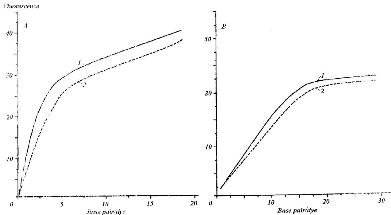
Fig. 3. Fluorescence titration of Cyan 6—Trp (1) and Cyan 6—Tyr (2) with DNA (A) and RNA (B). Fluorescence intensity is in arbitrary units.
