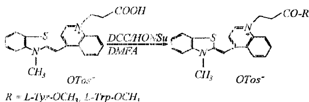
Fig. 1. Synthetic scheme of preparation of dye—amino acid conjugates
