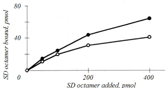
Fig. 2. Kinetics of binding between [ ^{32} P]oct and 30S RSUs vs. that of binding between [ ^{32} P]oct and 70S ribosomes. One hundred pmoles of 30S RSUs or 70S ribosomes were incubated with 50 to 400 pmoles of [ ^{32} P]oct. The radioactivity bound to 30S RSUs (filled circles) and 70S ribosomes (empty circles) was detected after their centrifuging through sucrose gradient. The values represent the mean of three experiments
