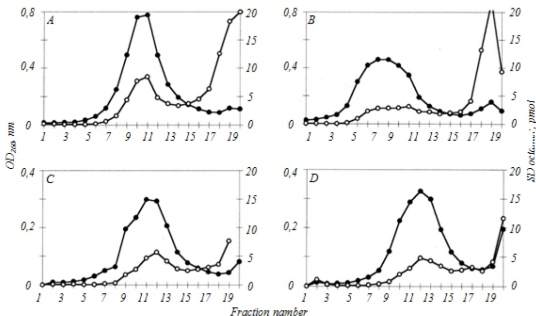
Fig. 5. Interaction of [ 32 P]oct with 70S ribosomes and its competition with 002 mRNA. The analysis through sucrose gradient was performed as for Fig. 4. (A) Incubation of 100 pmol of 70S ribosomes with 200 pmol of [ 32 P]oct. (B) Incubation of 100 pmol of 70S ribosomes with 200 pmol of [ 32 P]oct and 200 pmol of unlabelled mRNA (competition of [ 32 P]oct with mRNA for the binding with the 70S ribosomes). (C) Incubation of 100 pmol of 70S ribosomes with 200 pmol of [ 32 P]oct, 200 pmol of unlabelled mRNA and 100 pmol of unlabelled fMet-tRNA (competition of [ 32 P]oct with mRNA for the binding with the 70S ribosomes in the presence of fMet-tRNA). (D) Incubation of 100 pmol of 70S ribosomes with 200 pmol of [ 32 P]oct, 200 pmol of unlabelled mRNA and 100 pmol of unlabelled fMet-tRNA and Phe-tRNA (competition of [ 32 P]oct with mRNA for the binding with the 70S ribosomes in the presence of fMet-tRNA and Phe-tRNA). Filled circles: OD at 260 nm. Empty circles: amount of the captured [ 32 P]oct. The experiments were repeated three times for (A) and two times for (B), (C), and (D)
