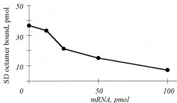
Fig. 3. Competition between [ ^{32} P]oct and 002 mRNA for binding with the anti-SD sequence of 16S rRNA. Fifty pmoles of 30S RSUs were incubated with 100 pmoles of [ ^{32} P]oct, in the presence of 0 to 100 pmoles of mRNA. The radioactivity bound to 30S RSUs was detected after centrifuging through sucrose gradient. The experiment was repeated twice
