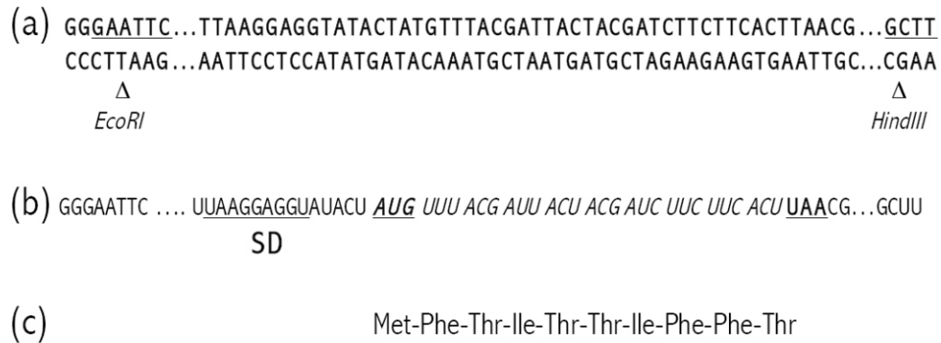
Fig. 1. Model 002 gene integrated in the plasmid pTZ18. (a) Double stranded DNA: the restriction sites for EcoRI and HindIII are underlined. (b) mRNA transcript: the SD sequence, the initiation codon AUG and the stop codon UAA are underlined; the «reading frame» is in italics. (c) Encoded peptide constituted by 10 residues. The dots, in (a) and (b), replace a number of upstream and downstream nucleotides not shown
