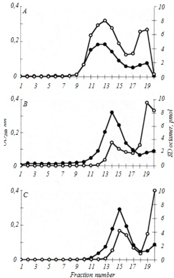
Fig. 4. Interaction of [ ^{32}\text{P} ]oct with 16S rRNA and its competition with 002 mRNA in the absence and in the presence of IFs and fMet-tRNA. A 10–30% sucrose gradient was performed in Nierenberg buffer containing, in 10 mM Tris-HCl at pH 7.7, 10 mM magnesium acetate and 60 mM \text{NH}_4\text{Cl} at pH 7.7. Centrifuging through this gradient lasted 2 hrs at 40,000 rev./min in the rotor TST 60.4 of the Kontron. (A) Incubation of 100 pmol of 30S RSUs with 200 pmol of [ ^{32}\text{P} ]oct. (B) Incubation of 50 pmol of 30S RSUs with 100 pmol of [ ^{32}\text{P} ]oct and 100 pmol of unlabelled mRNA. (C) Incubation of 50 pmol of 30S RSUs with 100 pmol of [ ^{32}\text{P} ]oct, 100 pmol of unlabelled mRNA and 50 pmol of unlabelled IF _1 , IF _2 , IF _3 , and fMet-tRNA. The fractions were 200 \mu\text{l} each: the first corresponded to the bottom of the centrifuge tube; the last corresponded to its top. Filled circles: OD at 260 nm. Empty circles: amount of the captured [ ^{32}\text{P} ]oct. The experiments were repeated three times for (A) and two times for (B) and (C)
