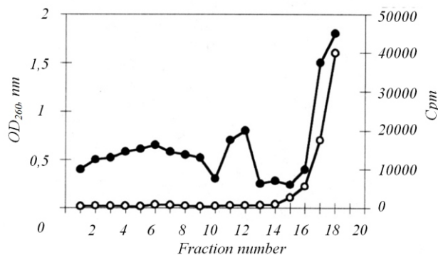
Fig. 6. Interaction between [ 32 P]oct and polysomes. 100 pmol of polysomes were incubated with 200 pmol of [ 32 P]oct. The analysis through sucrose gradient was performed as for Fig. 4 and 5. Filled circles: OD at 260 nm. Empty circles: radioactivity of captured [ 32 P]oct. The experiment was repeated twice
