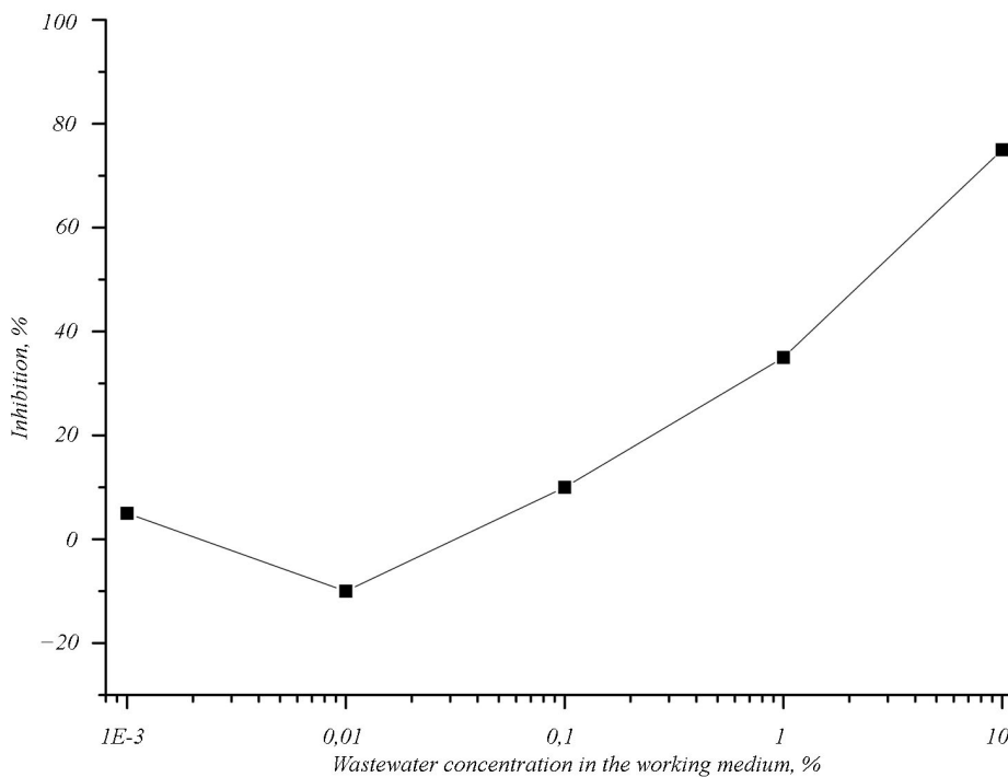
Fig. 7. Evolution of alkaline phosphatase activity rate after exposure at different concentrations of wastewater detected with conductometric biosensor. Measurements were conducted in 1 mM Mg(NO 3 ) 2 with 10 mM Tris-nitrate buffer, pH 8.5
