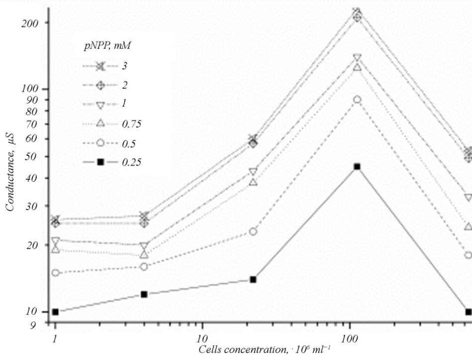
Fig. 2. Dependence of conductometric biosensor response on algal cells concentration in sol-gel membrane for different pNPP concentrations. Measurements were conducted in 1 mM \text{Mg}(\text{NO}_3)_2 with 10 mM Tris-nitrate buffer, pH
