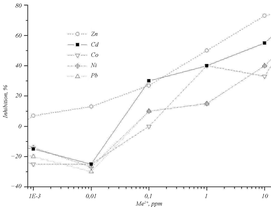
Fig. 6. Calibration curves of conductometric algal biosensor for different metal ions. Measurements were conducted in 1 mM Mg(NO 3 ) 2 with 10 mM Tris-nitrate buffer, pH 8.5
