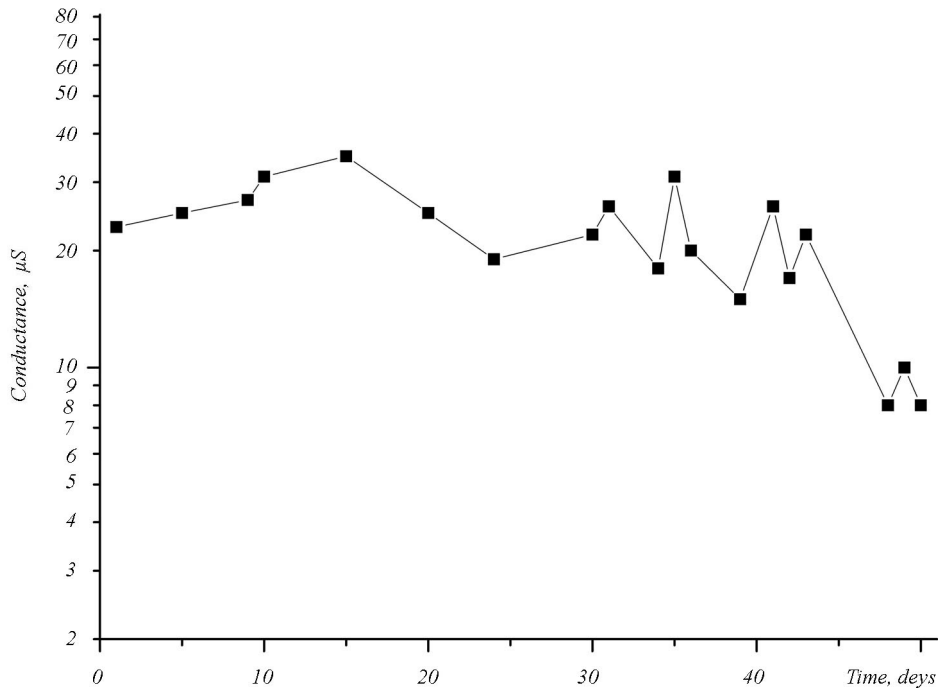
Fig. 5. Dependence of the algal biosensor response on storage life for 2 mM pNPP. Measurements were conducted in 1 mM Mg(NO_3)_2 with 10 mM Tris-nitrate buffer, pH 8.5
