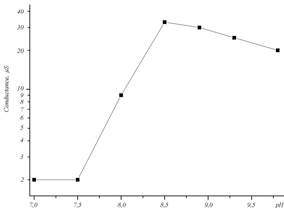
Fig. 3. pH-Dependence of conductometric biosensor response for 2 mM of pNPP. Measurements were conducted in 1 mM Mg(NO_3)_2 with 10 mM Tris-nitrate buffer, pH 8.5
