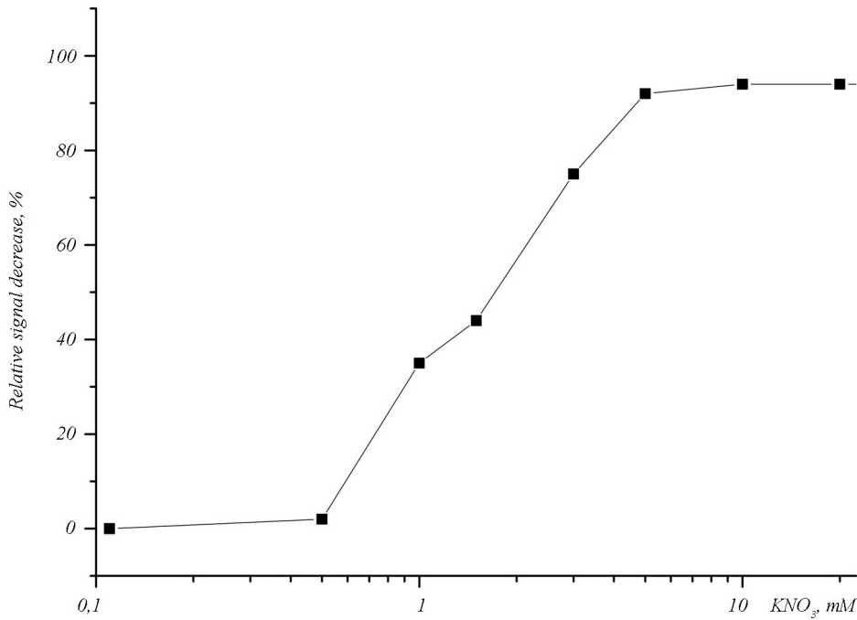
Fig. 4. Dependence of conductometric biosensor relative signal decrease on ionic strength for 2 mM pNPP. Measurements were conducted in 1 mM Mg(NO_3)_2 with 10 mM Tris-nitrate buffer, pH 8.5
