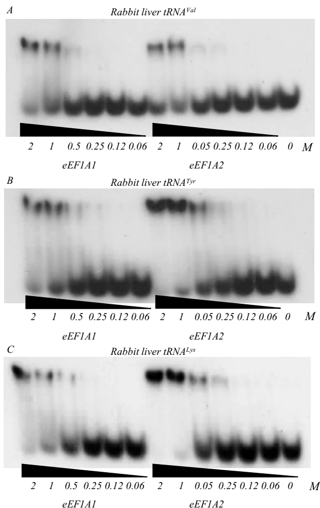
Fig. 1. The stability test for ternary complexes of tRNAs with eEF1A1*GDP and eEF1A2*GDP: A – Radioautograph of electrophoregram of eEF1A1*GDP*tRNA Val and eEF1A2*GDP*tRNA Val complexes at eEF1A1/eEF1A2 concentration range from 2 M to 0.06 M, in non-denaturing (native) conditions; B – like A but eEF1A1*GDP*tRNA Tyr and eEF1A2*GDP*tRNA Tyr complexes; C – like A but eEF1A1*GDP*tRNA Lys and eEF1A2*GDP*tRNA Lys complexes
