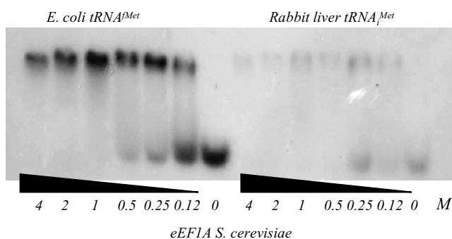
Fig. 3. Stability test of the complexes eEF1A from S. cerevisiae with deacylated tRNA^{fMet} from E. coli and tRNA_i^{Met} from rabbit liver
