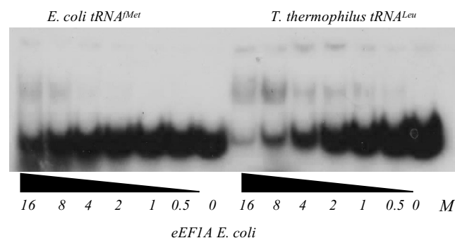
Fig. 4. Band Shift Assay of eEF1A from E. coli with tRNA_f^{Met} from E. coli and tRNA^{Leu} from T. thermophilus
