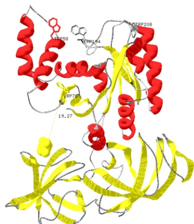
Fig. 5. Model of S. cerevisiae eEF1A (adopted from [41]) based on the X-ray structure of eEF1A in complex with eEF1B (truncated eEF1B hidden), hypothetical location of C74 shown and traced to Trp78 of eEF1A
