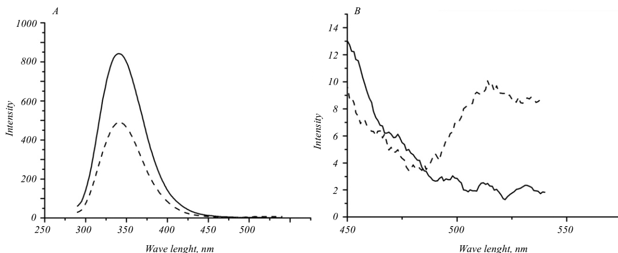
Fig. 6. A – Measurement of FRET efficiency from Trp residue of yeast eEF1A to 1,5-IAEDANS covalently bound to the C74 of tRNA 3 Lys (solid lines show internal fluorescence of 500 nm eEF1A, dashed lines show decrease in fluorescence intensity in presence of equal amount of labeled tRNA 3 Lys ); B – a magnified area of 1,5-IAEDANS emission maximum where FRET was observed
