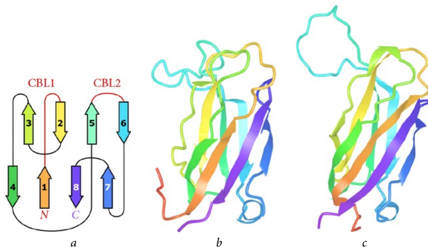
Fig. 4. Tertiary structure prediction of C2 domain of Bcr. a — schematic representation of II type topology of C2 domains, b — structure predicted with DMPfold, c — structure predicted with AlphaFold
