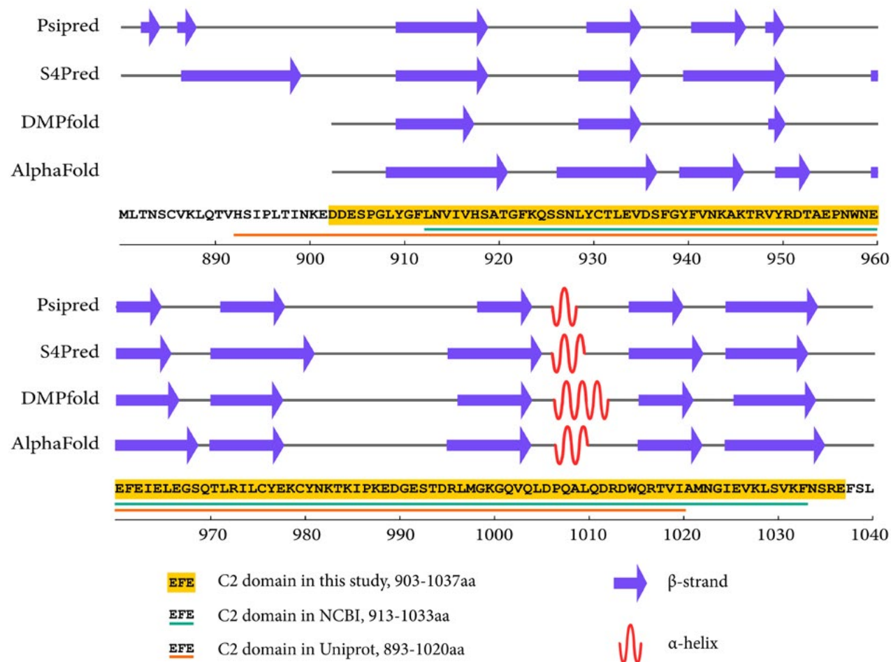
Fig. 3. Prediction of secondary structure of C2 domain of Bcr
